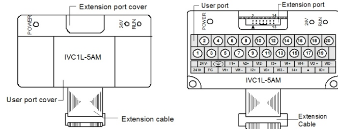
Figure 1-1 IVC1L-5AM appearance Figure 1-2 IVC1L-5AM Ports
