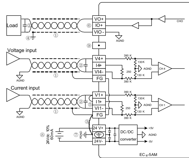
Figure 1-4 Wiring of IVC1L-5AM user port
