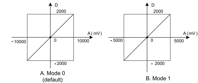
Figure 3-2 Default input channel characteristics in various modes
