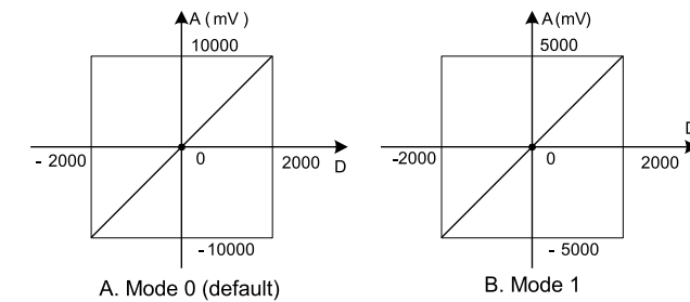
Figure 3-5 Default output channel characteristics in various modes
