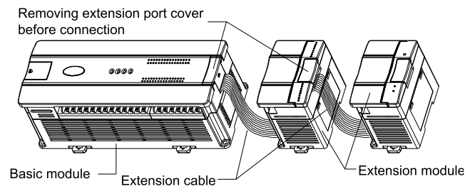
Figure 1-3 Connecting IVC1L-5AM to the basic module
