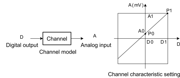
Figure 3-4 IVC1L-5AM output channel characteristic
