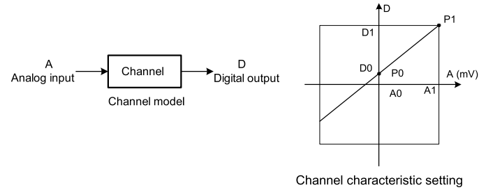
Figure 3-1 IVC1L-5AM input channel characteristic
