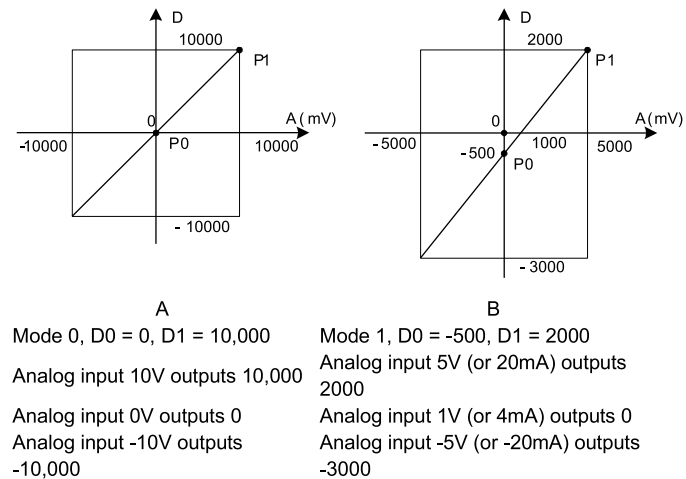
Figure 3-3 Changing input channel characteristics
