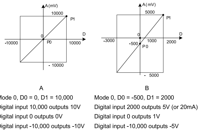
Figure 3-6 Changing output channel characteristics
